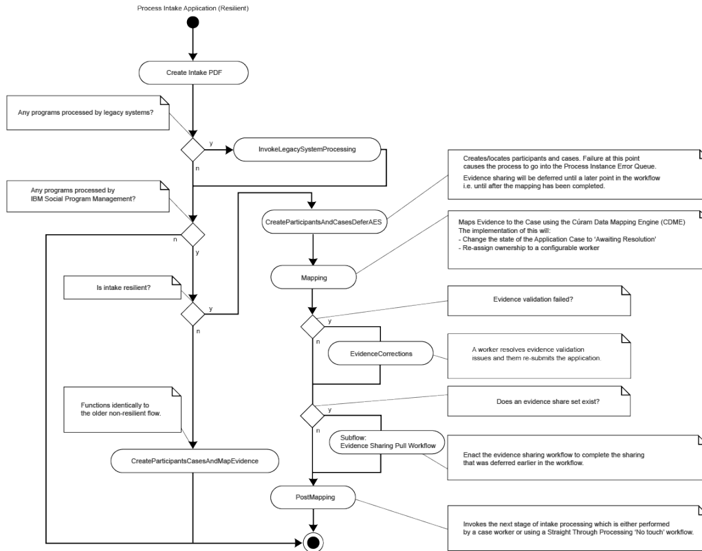
Figure 5. Intake application workflow
